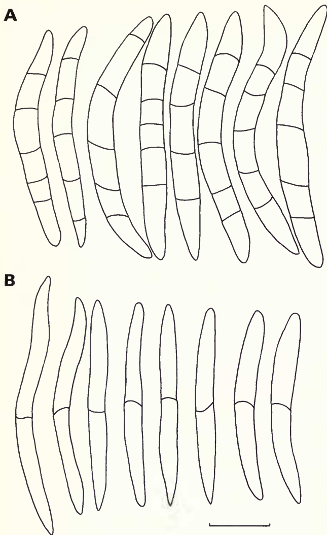
Fig. 16 Ascospore outlines (A) Leptorhaphis oleae (Massal.) Körber (VER-holotype); (B) Leptorhaphis parameca (Massal.) Körber (VER-holotype); scale = 10 \mu m.
